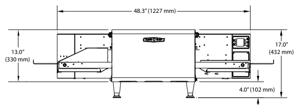
Figure 3: Oven Dimensions - Front (Single)
